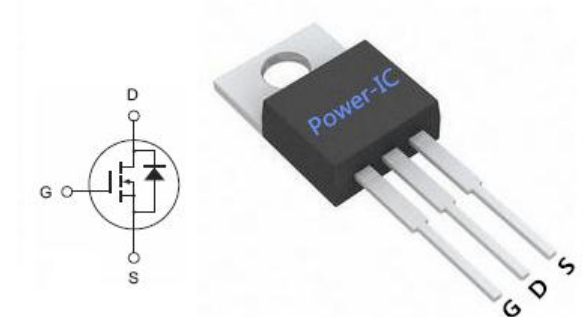
TO-220 Package
